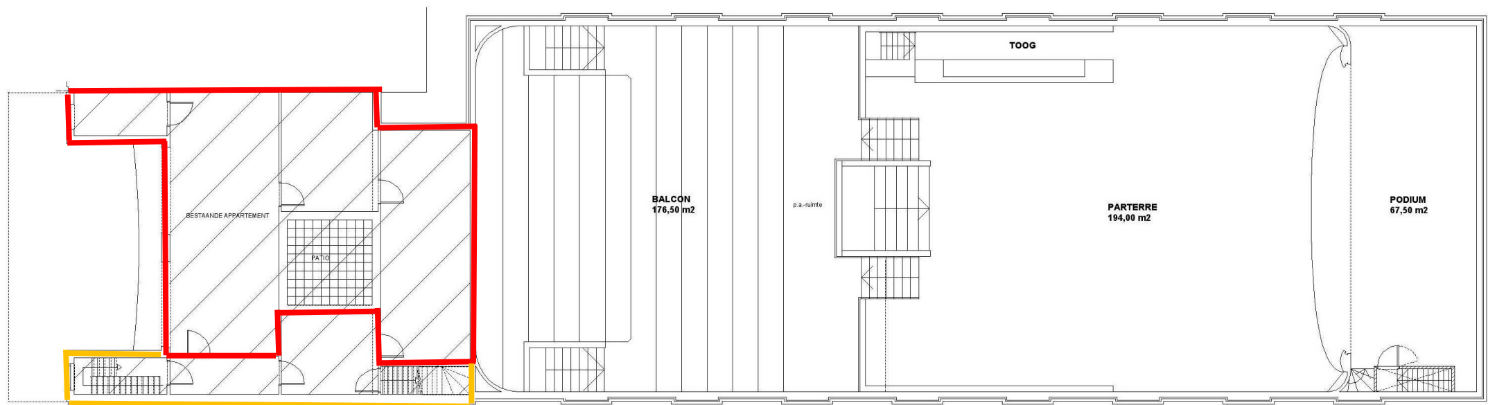
PLAN VERDIEPING 1
